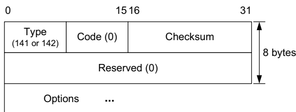
Figure 8-36 The ICMPv6 IND Solicitation (type 141) and Advertisement (type 142) messages have the same basic format. They are used to map known link-layer addresses to IPv6 addresses in environments where this is useful.
